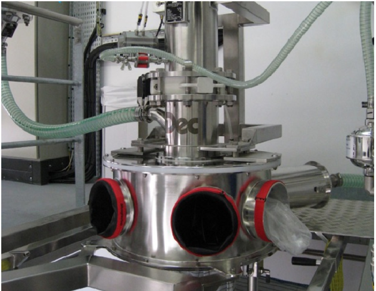
Dec DCS high containment drum and big bag filling
